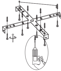
2. Drill holes & apply plastic Anchors with screws
