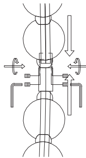
8. By rotating apply the screws
