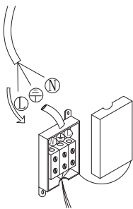
4. Connect the wires
