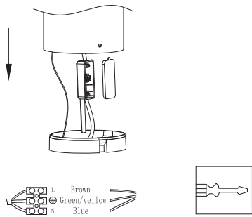
Connect wires
