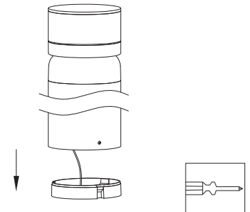
Remove from the base
