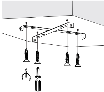
5. Apply screws
