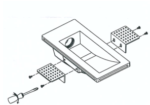
Untight the side screws
