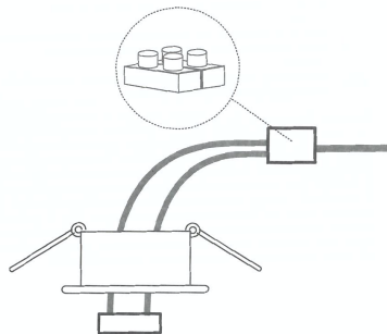
3. Connect wires
