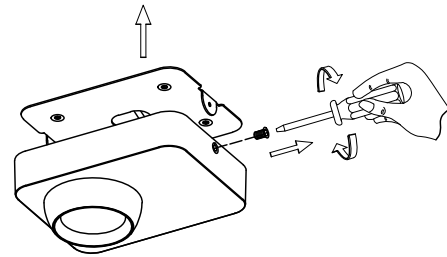
2. Untight the side screws
