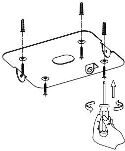
3. Drill holes & apply plastic anchors With screws
