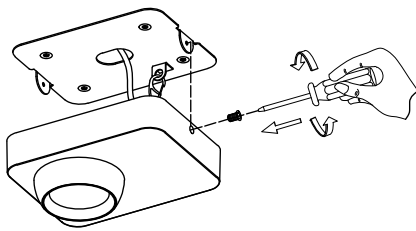
5. Apply the side screws
