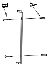
3. Apply plastic anchors with screws
