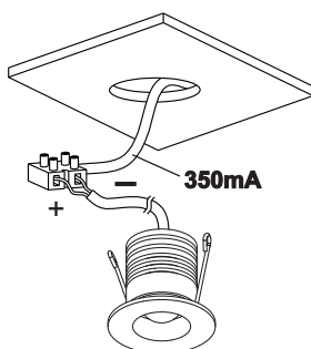
Connect wires
