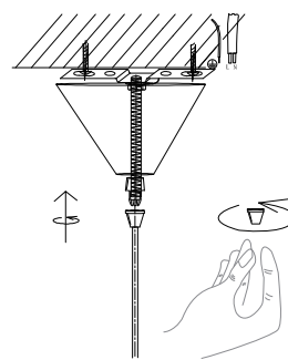
4 By Rotating Apply the cap
