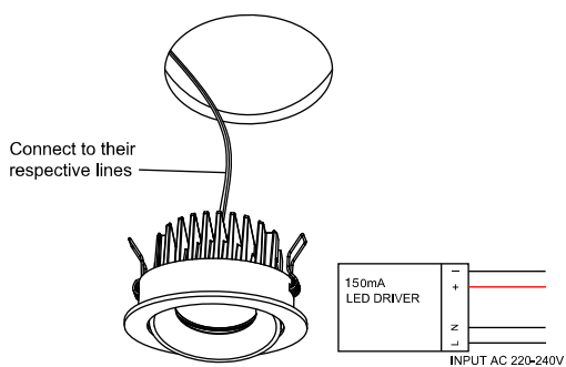
Connect the wires of the driver
