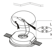
Connect the wires
