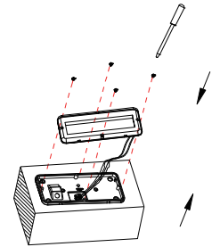
10. Install the PC cover.
