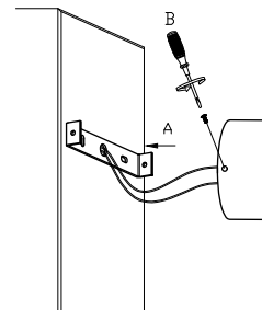
6 Apply the side screws
