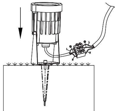
4. Connect wires & place the lamp into the ground
